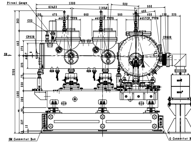
Monochromator of BOREAS beamline
